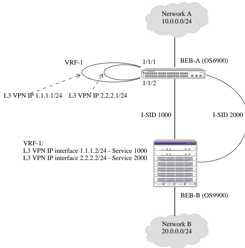
Figure 10: L3 VPN Loopback and Service-based Interfaces
