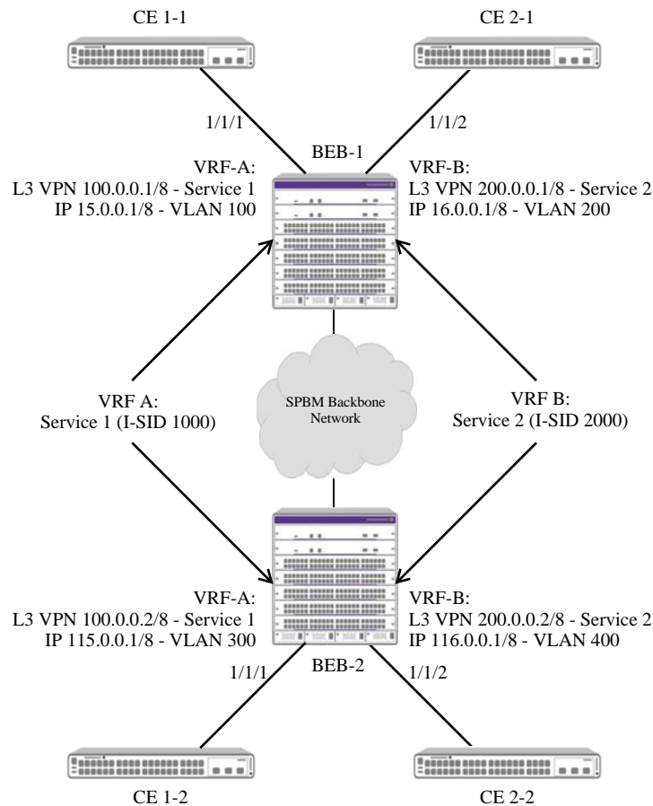
Figure 11: L3 VPN Service-based Interfaces
