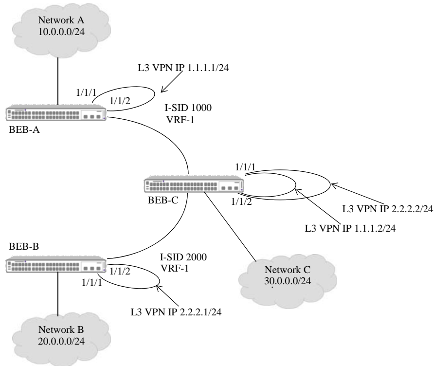
Figure 12: Inter-ISID Routing Example (One VRF)
