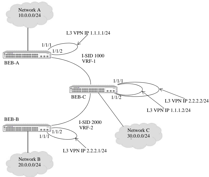
Figure 13: Inter-ISID Routing Example (Two VRFs)
