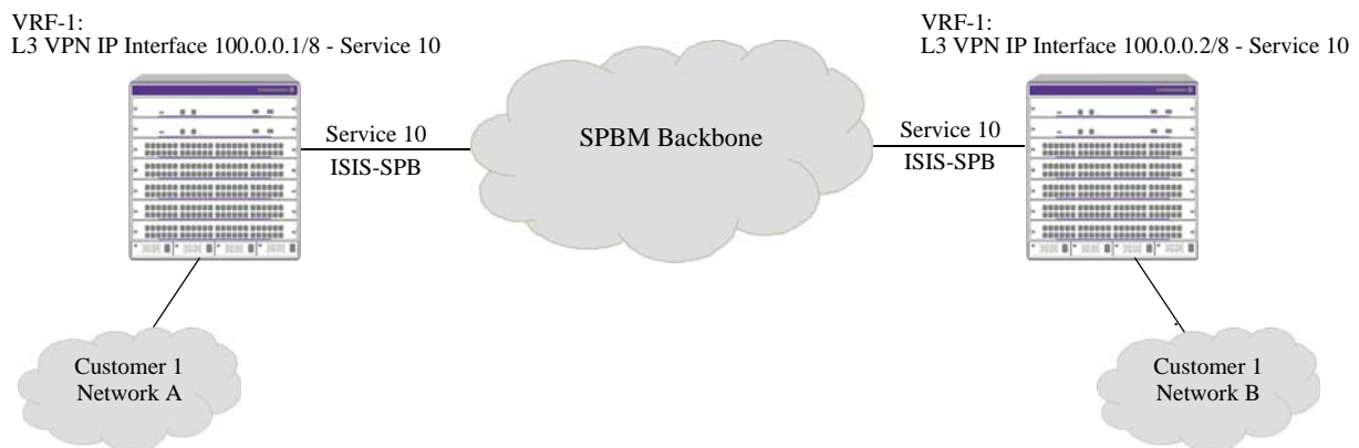
Figure 7: L3 VPN Interface (No Loopback)
